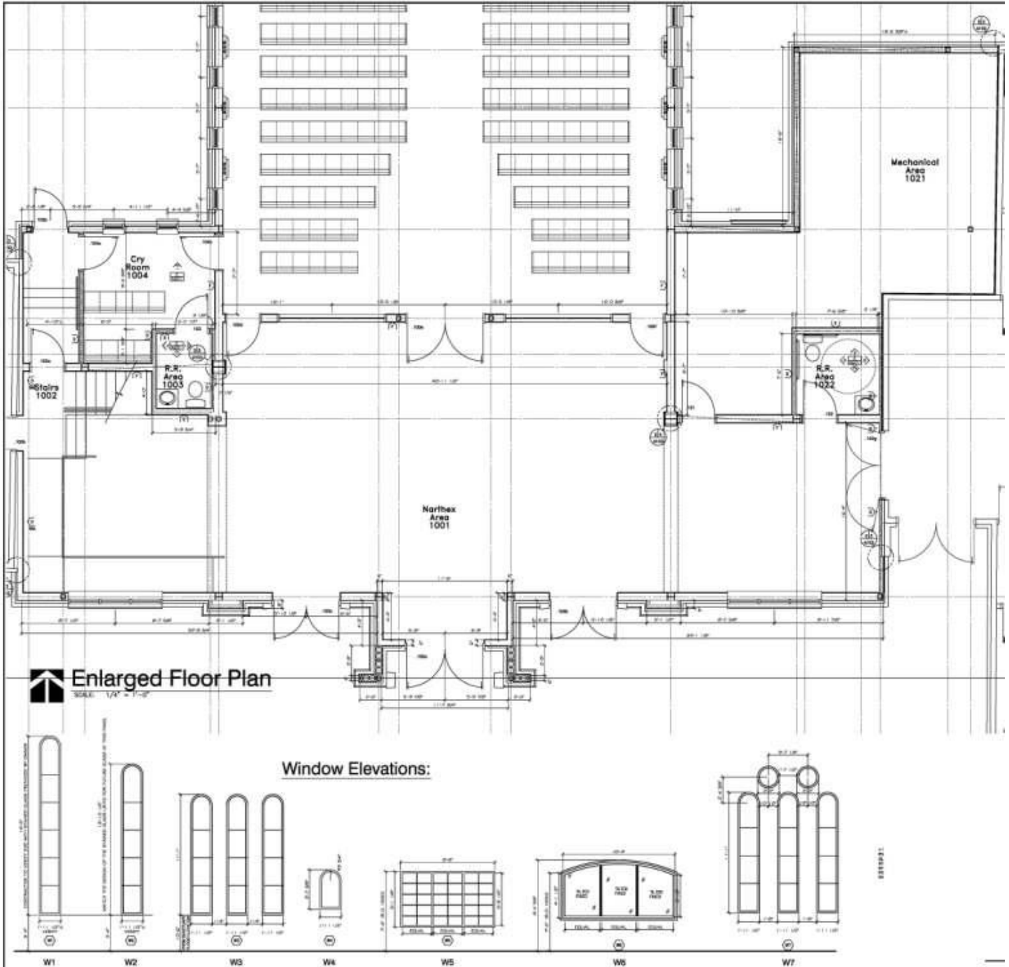
Floor plan of Church
